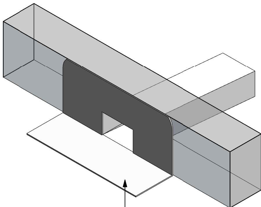
Viking Roofspec Scupper 01 M15: Scuppers - 100mm x 65mm C Viking Roofspec 100x65mm TPO scupper STP601, installed as per manufacturers instructions.
