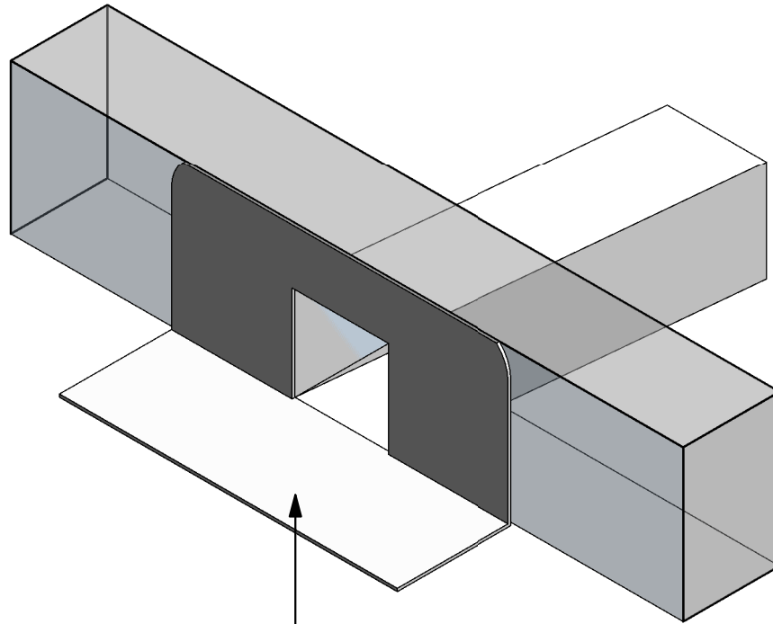
Viking Roofspec Scupper 02 M15: Scuppers - 100mm x 100mm A Viking Roofspec 100x100mm TPO scupper STP602, installed as per manufacturers instructions.
