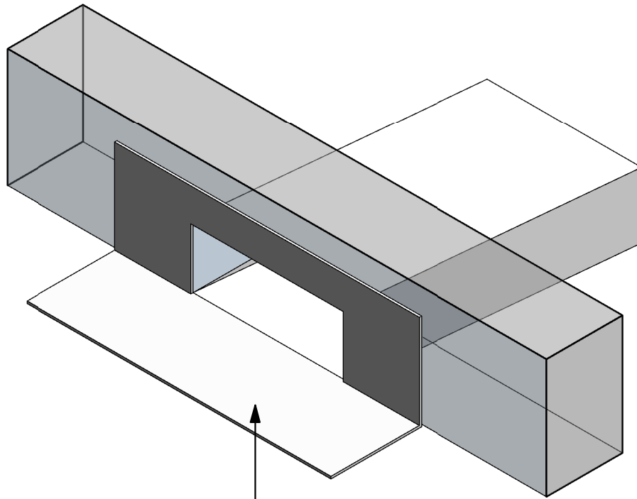
Viking Roofspec Scupper 03 M15: Scuppers - 200mm x 80mm Viking Roofspec 200x80mm TPO scupper STP603, installed as per manufacturers instructions.
